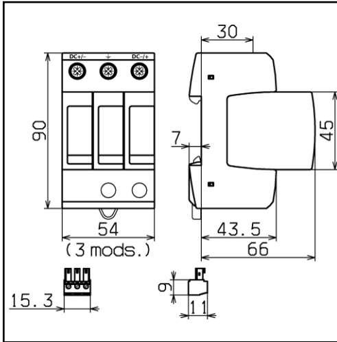
Dimension drawing DG M YPV SCI 600 FM
