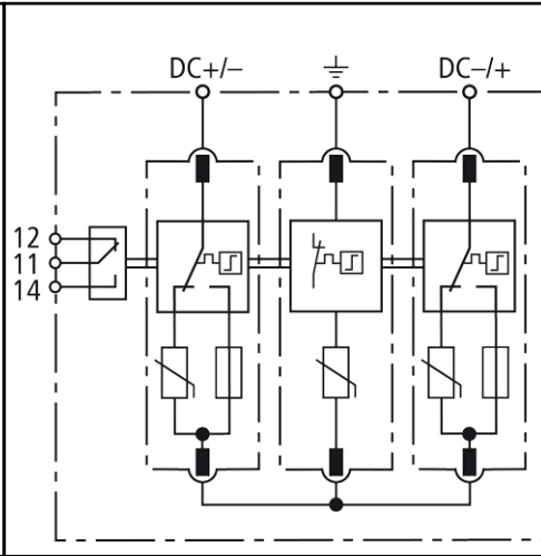
Basic circuit diagram DG M YPV SCI 600 FM
